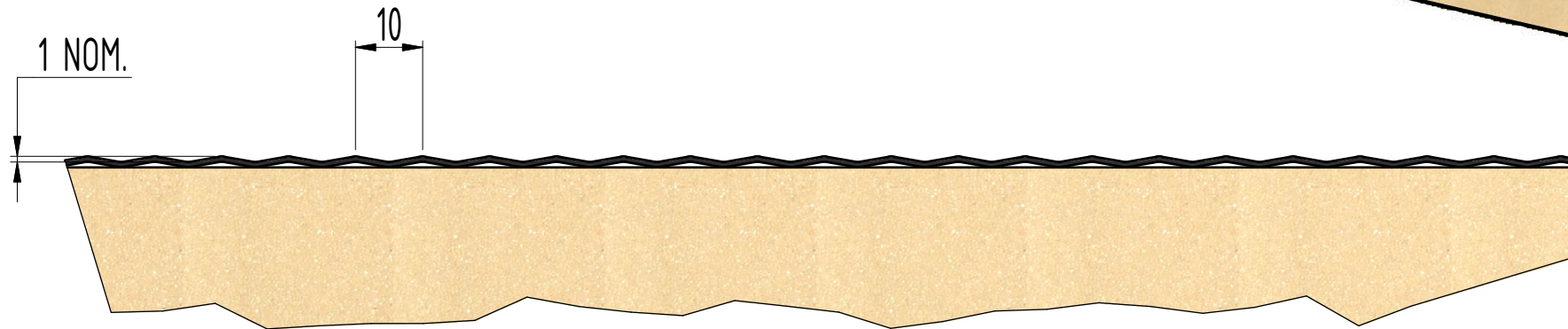
DETAIL B
